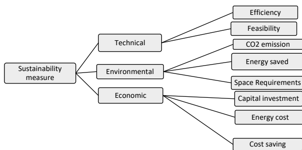
Figure 4. MCDA framework.
